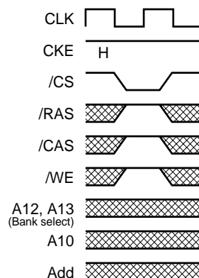
Fig.9 No operation
